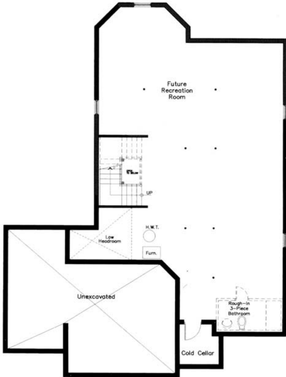
Basement Plan
