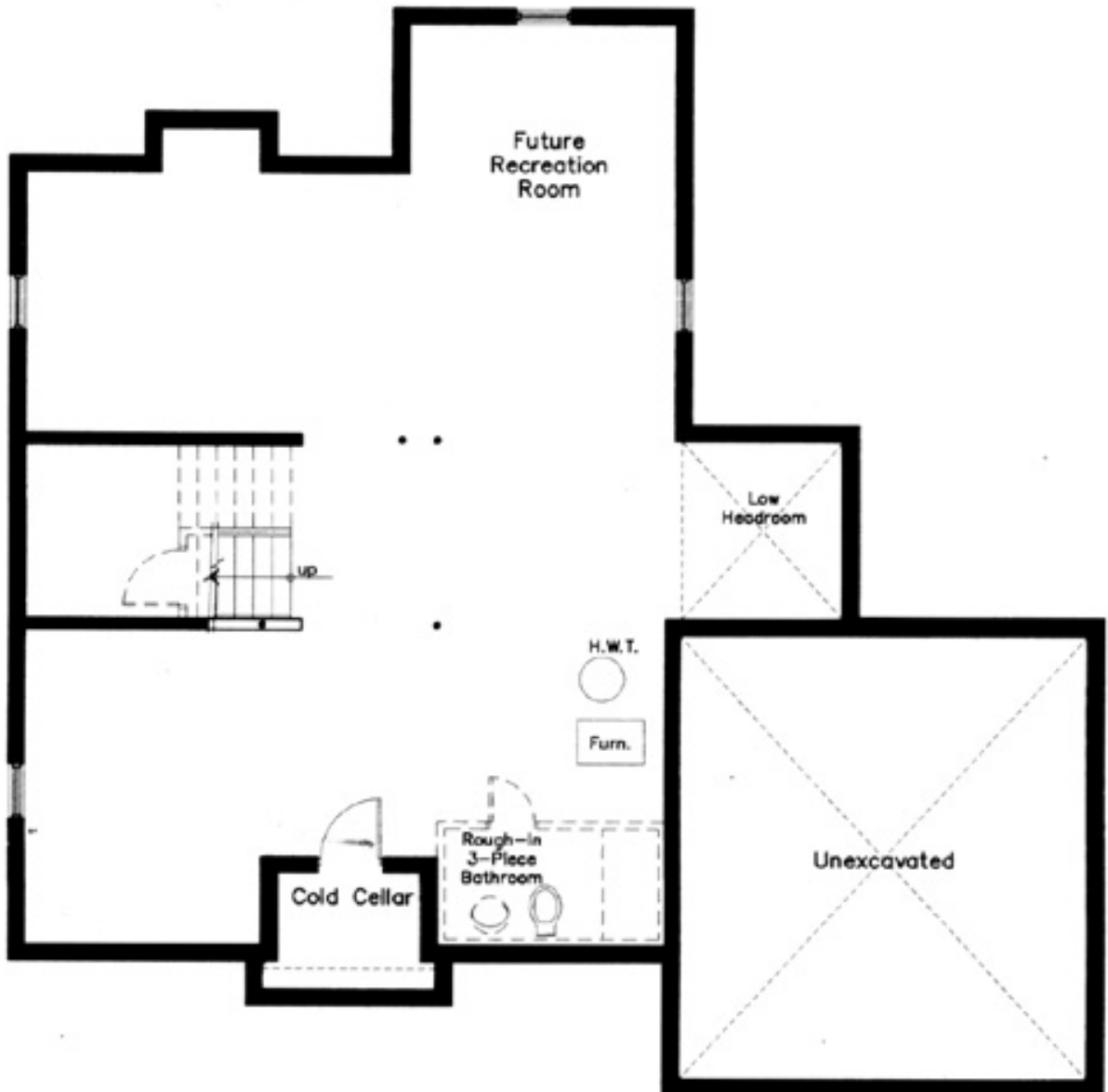
Basement Plan
