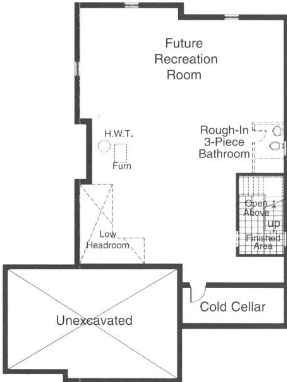
Basement Plan
