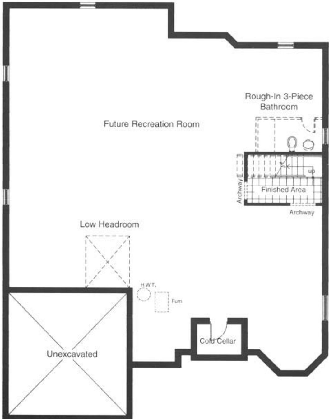
Basement Plan
